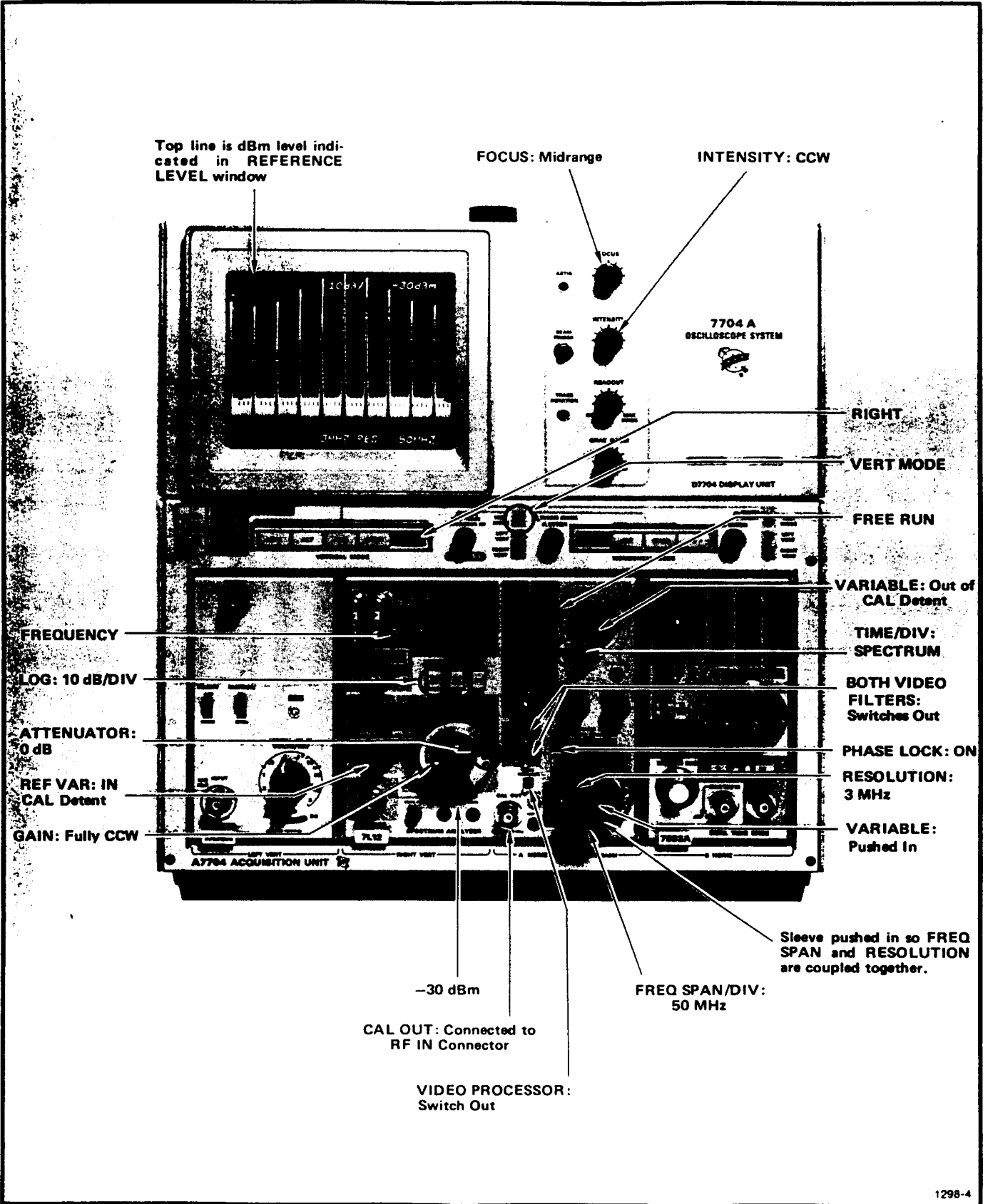
Fig. 2-2. 7L12 Spectrum Analyzer in a 7000-Series Oscilloscope illustrating initial settings of front panel controls and selectors. Circled (O) push-buttons denote button depressed or position of selector.
